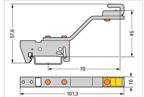
Busbar carrier; for (10 x 3) mm copper busbars; single side; angled; snaps onto DIN-35 rail
