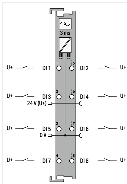
8-Channel Digital Input; 24 VDC; 3 ms
