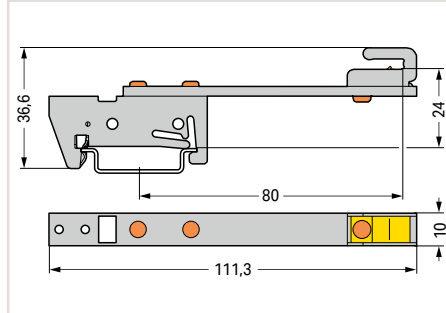
Busbar carrier; for (10 x 3) mm copper busbars; single side; straight; snaps onto DIN-35 rail
