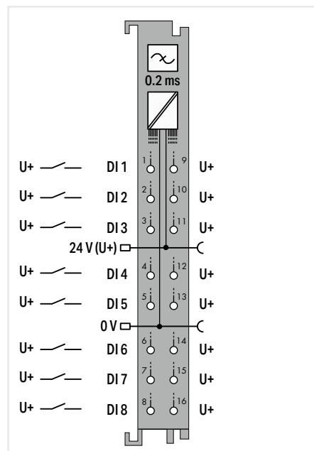
8-Channel Digital Input; 24 VDC; 0.2 ms; 2-wire connection
