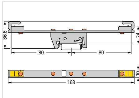
Busbar carrier; for (10 x 3) mm copper busbars; both sides; straight; snaps onto DIN-35 rail
