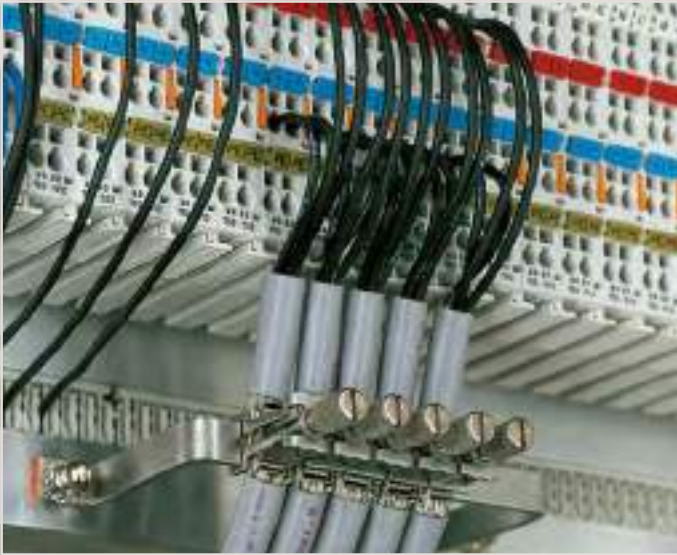
U-shaped (10 x 3) mm copper busbar
