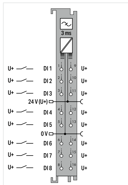
8-Channel Digital Input; 24 VDC; 3 ms; 2-wire connection
