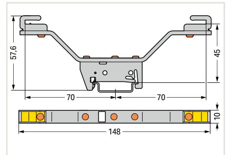
Busbar carrier; for (10 x 3) mm copper busbars; both sides; angled; snaps onto DIN-35 rail
