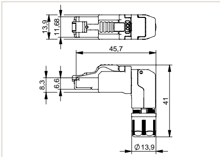
ETHERNET Connector; RJ-45; Cat. 6A; Angled; Code T568B; Strain relief
